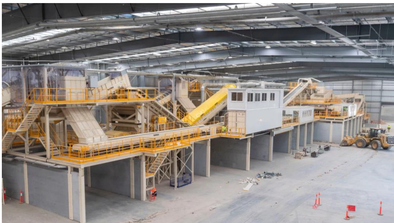
Mechanical sorting equipment at Wetherill Park prior to commissioning. Image courtesy of ResourceCo.
