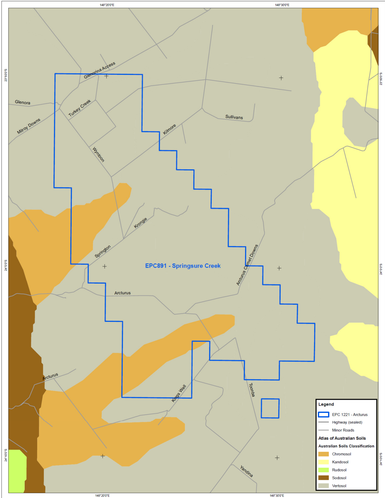
Figure 4. EPC 891 Springsure Creek - Soils
