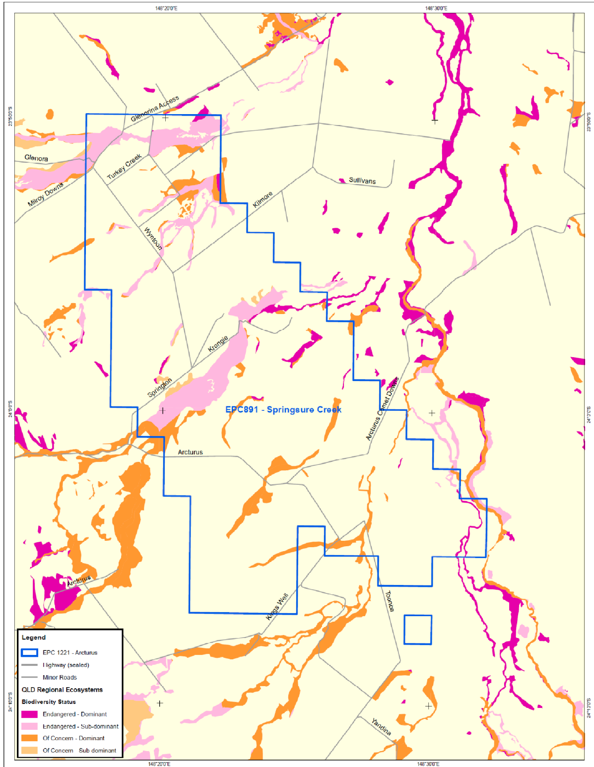
Figure 6. EPC 891 Springsure Creek - Regional Ecosystems
