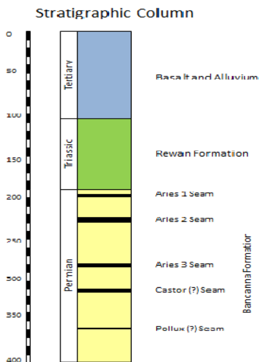
Figure 2. Stratigraphic Column for the Springsure Creek Deposit.
