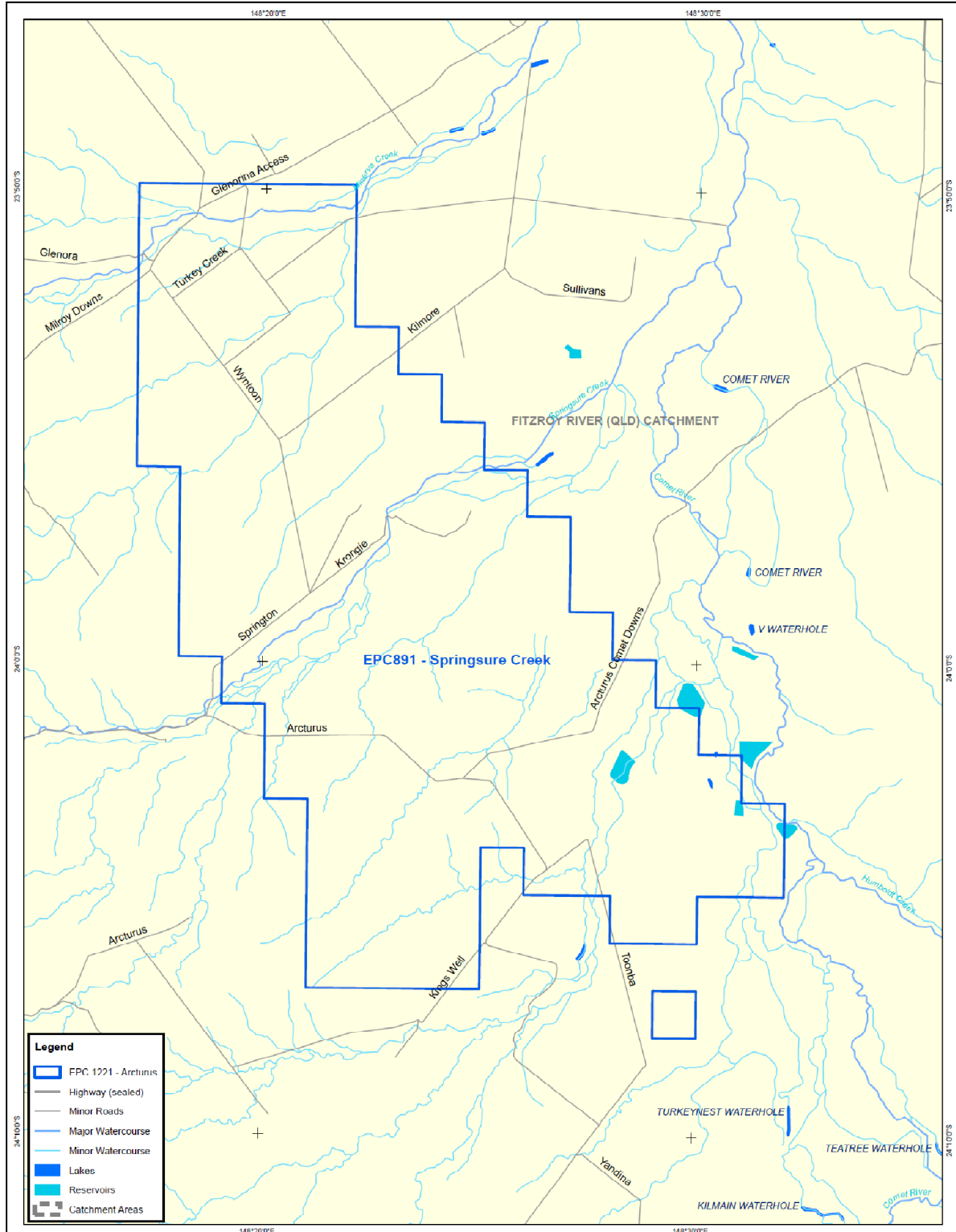
Figure 5. EPC 891 Springsure Creek - Hydrology
